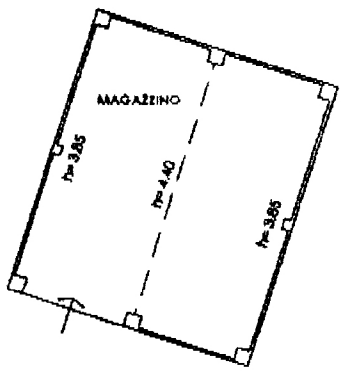
PIANO TERRENO
